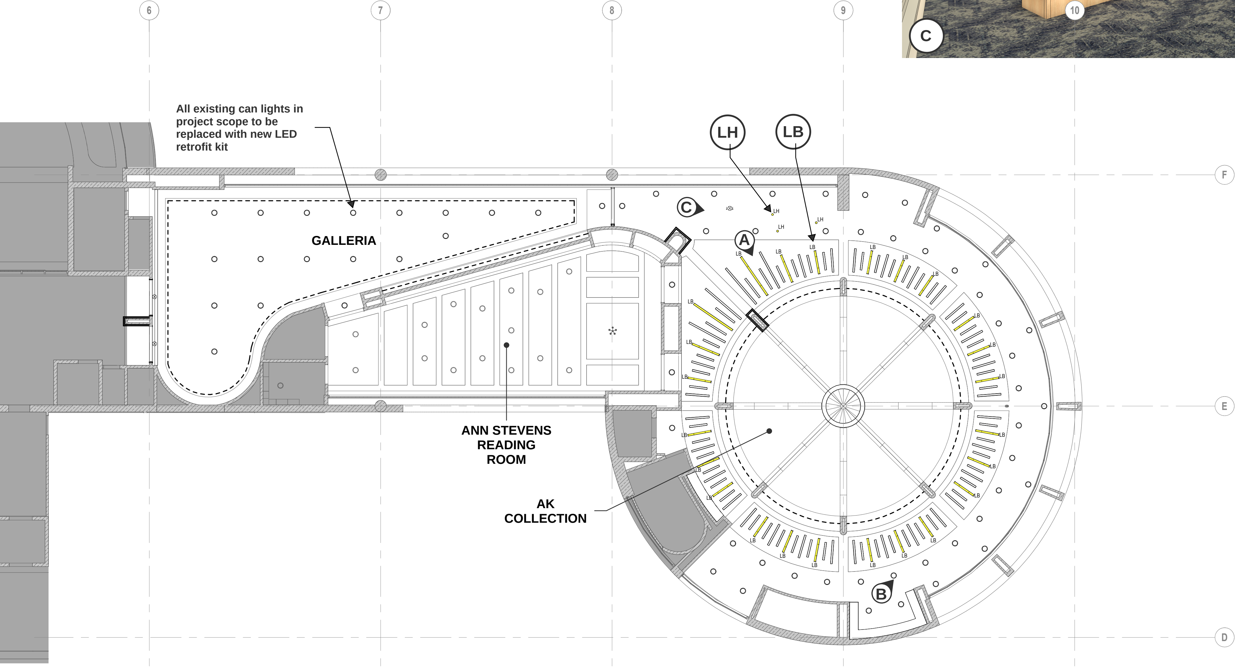
THIRD FLOOR REFLECTED CEILING PLAN
