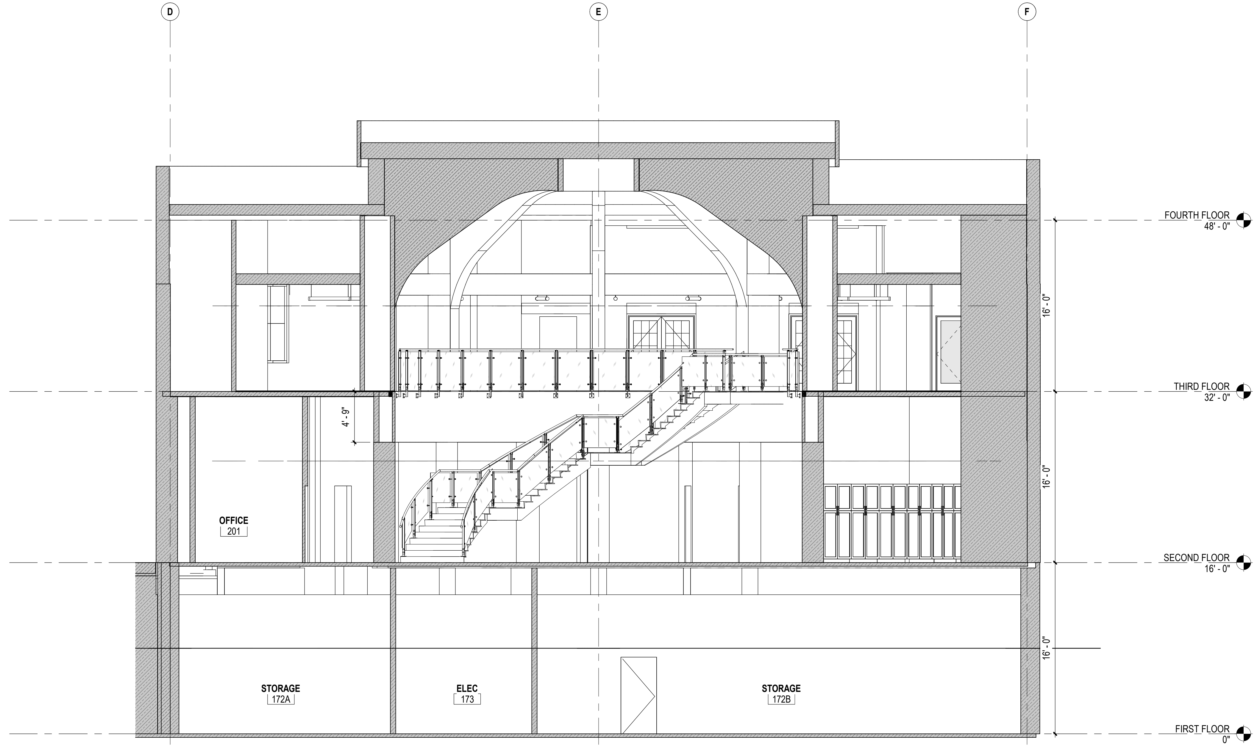
1 NORTH/SOUTH SECTION A301 3/16" = 1'-0"
